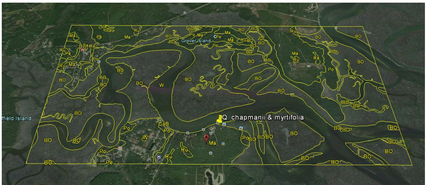
Soil map and potential specimen localities overlaid on an area near Crooked River State Park, Georgia.
